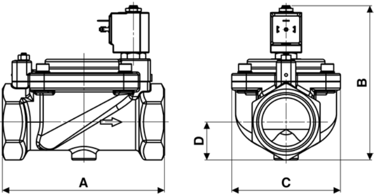
DIMENSIONS & WEIGHTS
