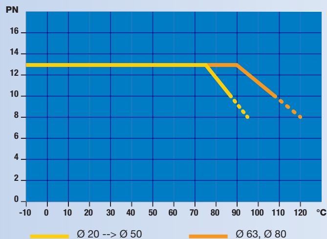
Curve showing compressed air pressure as a function of temperature
